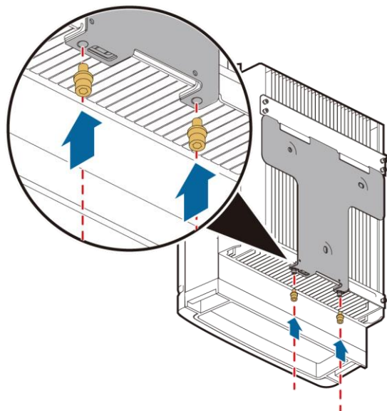
Figure 4-12 Tightening hexagon screws
