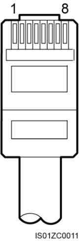
Figure 5-28 Connection sequence
