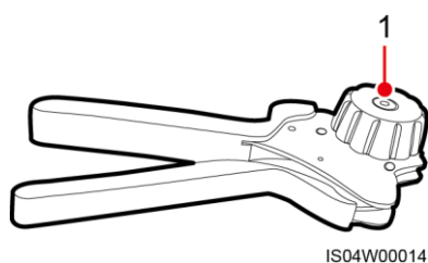
Figure 5-19 Crimping tool (H4TC0002)
